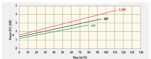
Power/Flow rate
