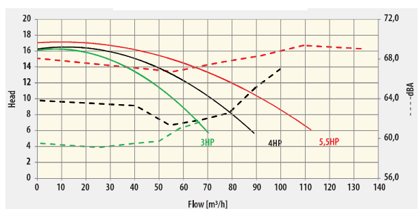
Pressure/Flow rate
