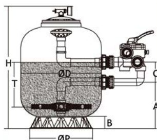
800-SM-2 ~ 900-SM-2
